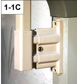
Post mounting bracket Telescope In / Out as required & Secure
