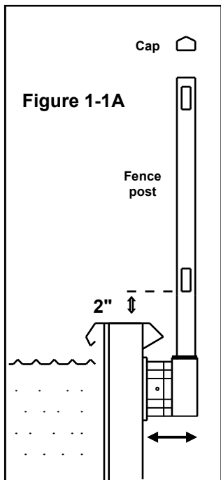
Post mounting bracket Telescope In / Out as required & Secure
