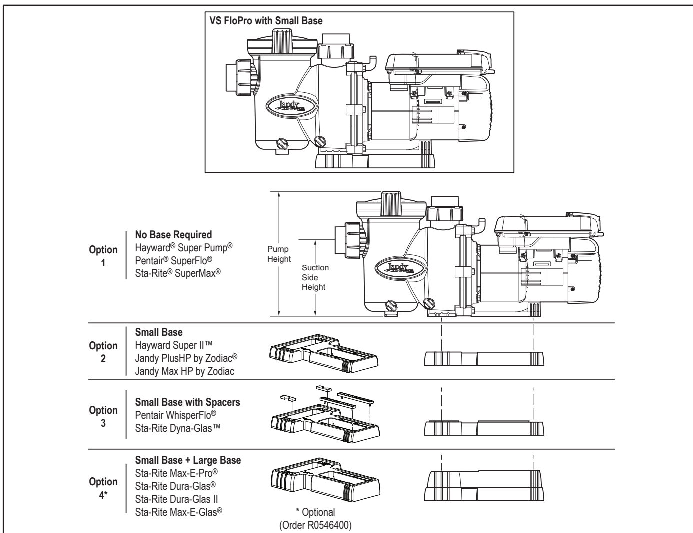
Figure 3. VS FloPro Pump and Base Options
