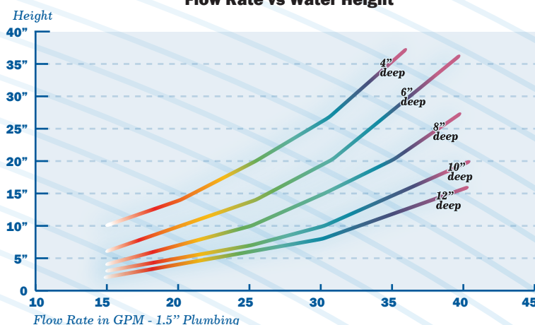
Flow Rate vs Water Height
