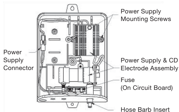
Figure 6 Internal component locations
