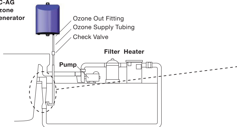
Figure 2 Installation Schematic for Injector Assembly
