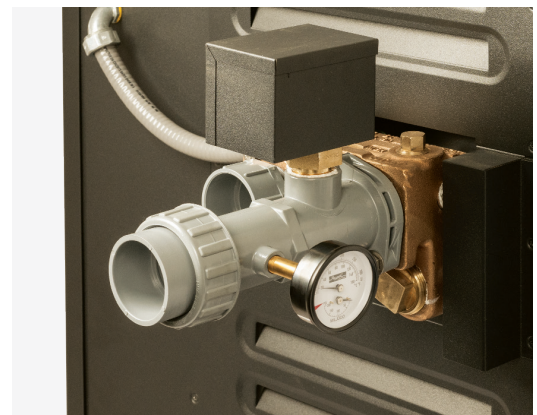
Flow switch and T&P gauge-standard
