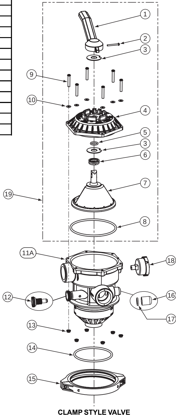
CLAMP STYLE VALVE
