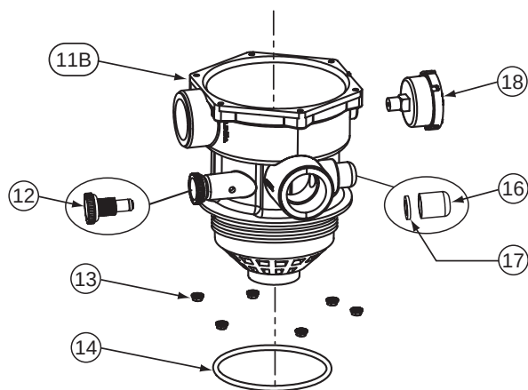
6" BUTTRESS STYLE VALVE
