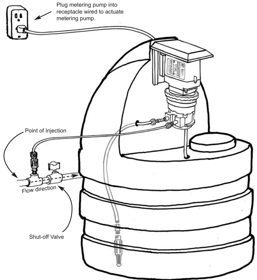
Stenner Pump/Tank system
