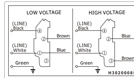
48SUP0753C-I, 48SUP1003C-I
