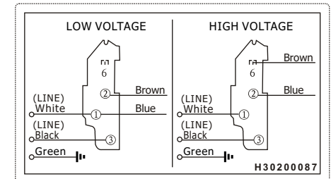
48SUP1653C-I
