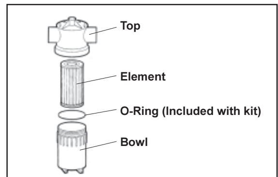
Figure 1. Energy Filter exploded view
