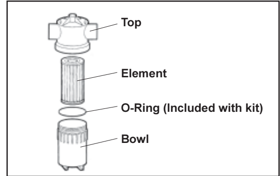
Figure 1. Energy Filter exploded view
