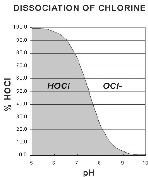
Figure 2 Equilibrium of Free Chlorine.
