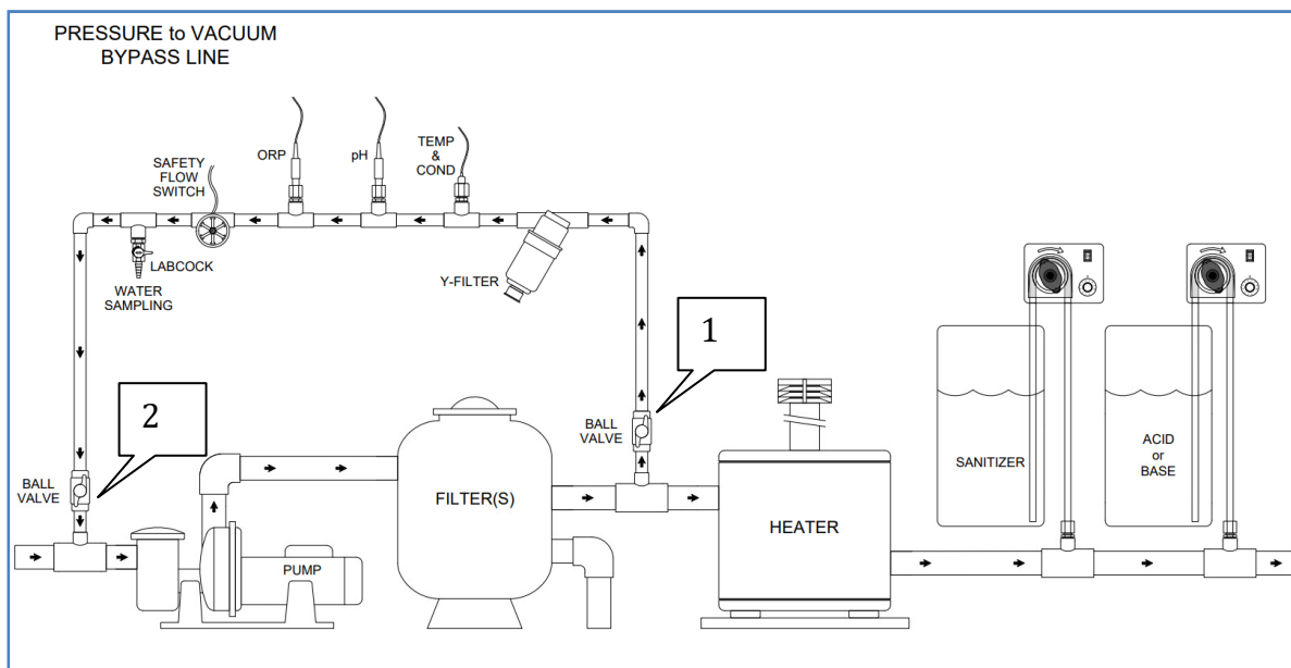
Figure 6. Pressure to Vacuum Bypass Line
