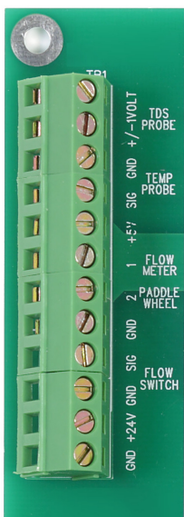
Figure 18. Sensor Connections on Power Board
