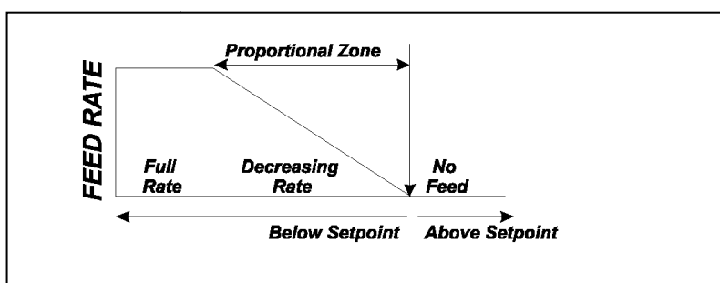
Figure 66. Proportional Feed Rate
