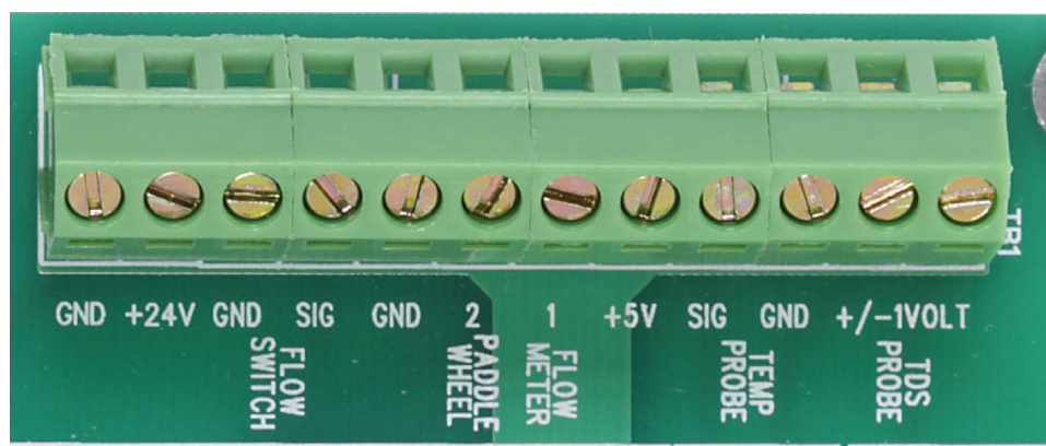
Figure 44. Connections to PC2100 (Power supply board)
