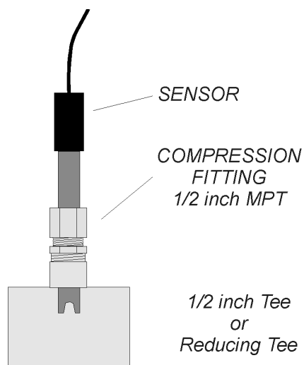
Figure 29. Sensor Installation
