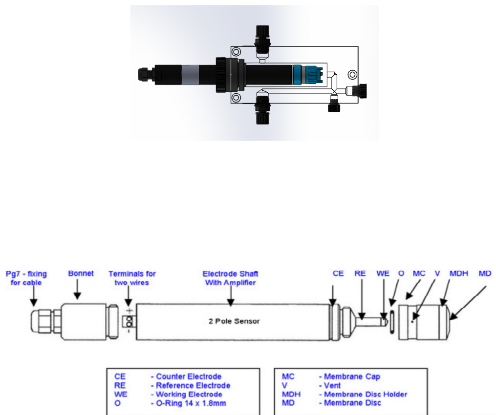
Figure 33. PPM Sensor and Mount
