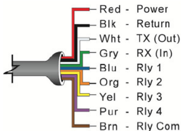
Figure 49. DX24 Wiring
