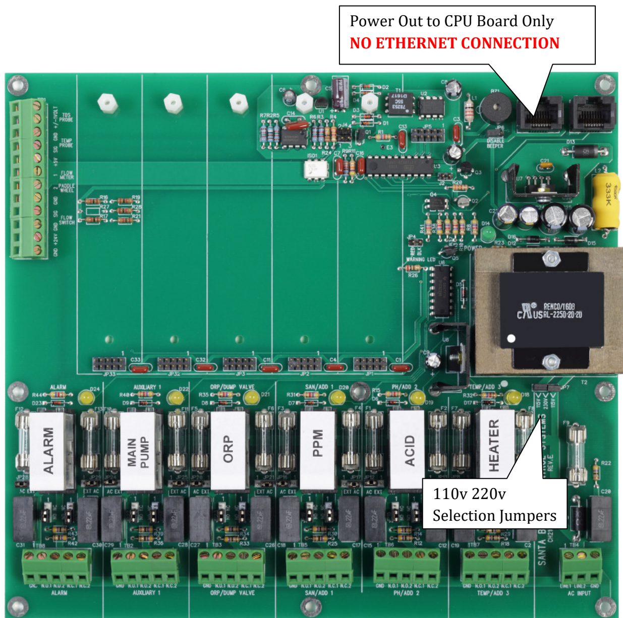
Figure 13. CH2100 Power Supply
