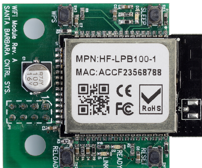
Figure 27. WiFi Adapter
