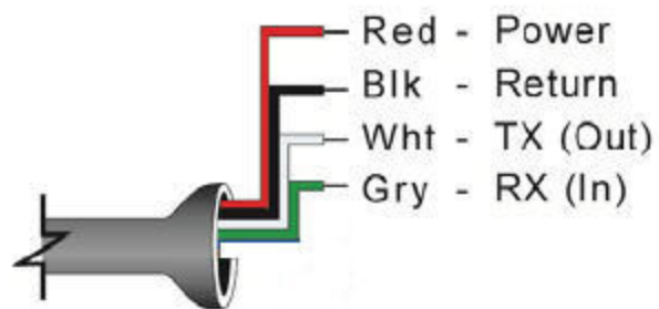
Figure 48. DX-10 Wiring
